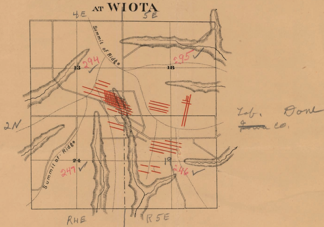
MAP OF ORE-BEARING CREVICES AT PORTERS GROVE
