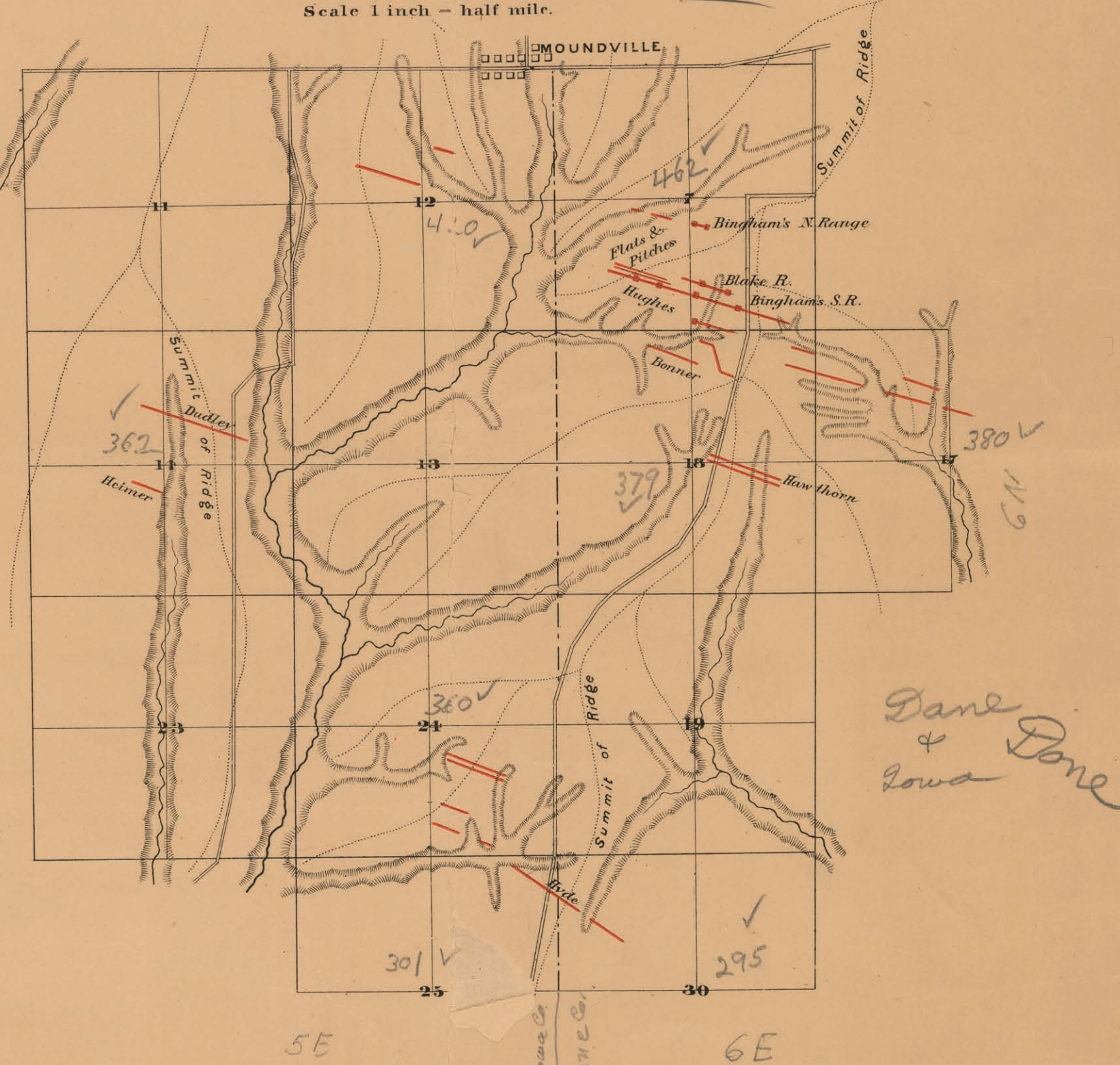
MAP OF ORE-BEARING CREVICES AT MOUNDVILLE
