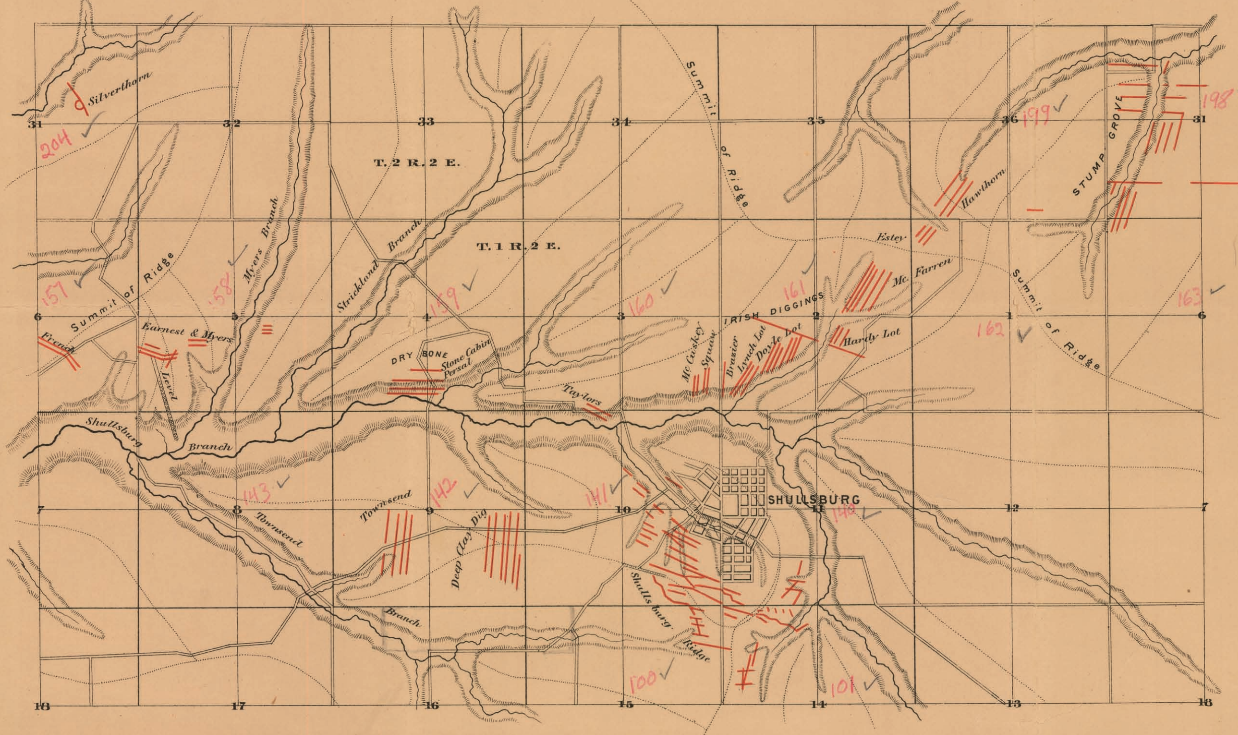
MAP OF ORE-BEARING CREVICES AT SHULLSBURG and VICINITY
