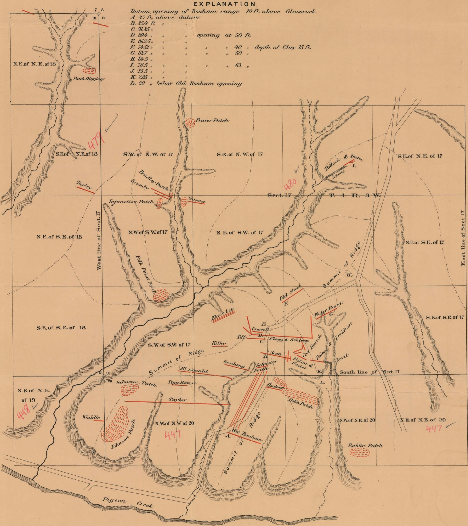
MAP OF ORE-BEARING CREVICES AT SHULLSBURG and VICINITY
