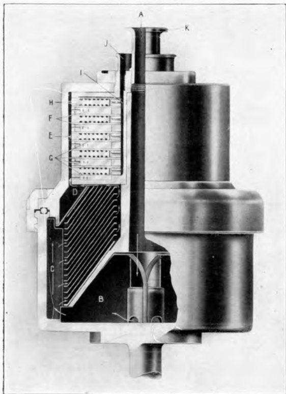
Fig. 4.—Sectional view of bowl of centrifuge.
