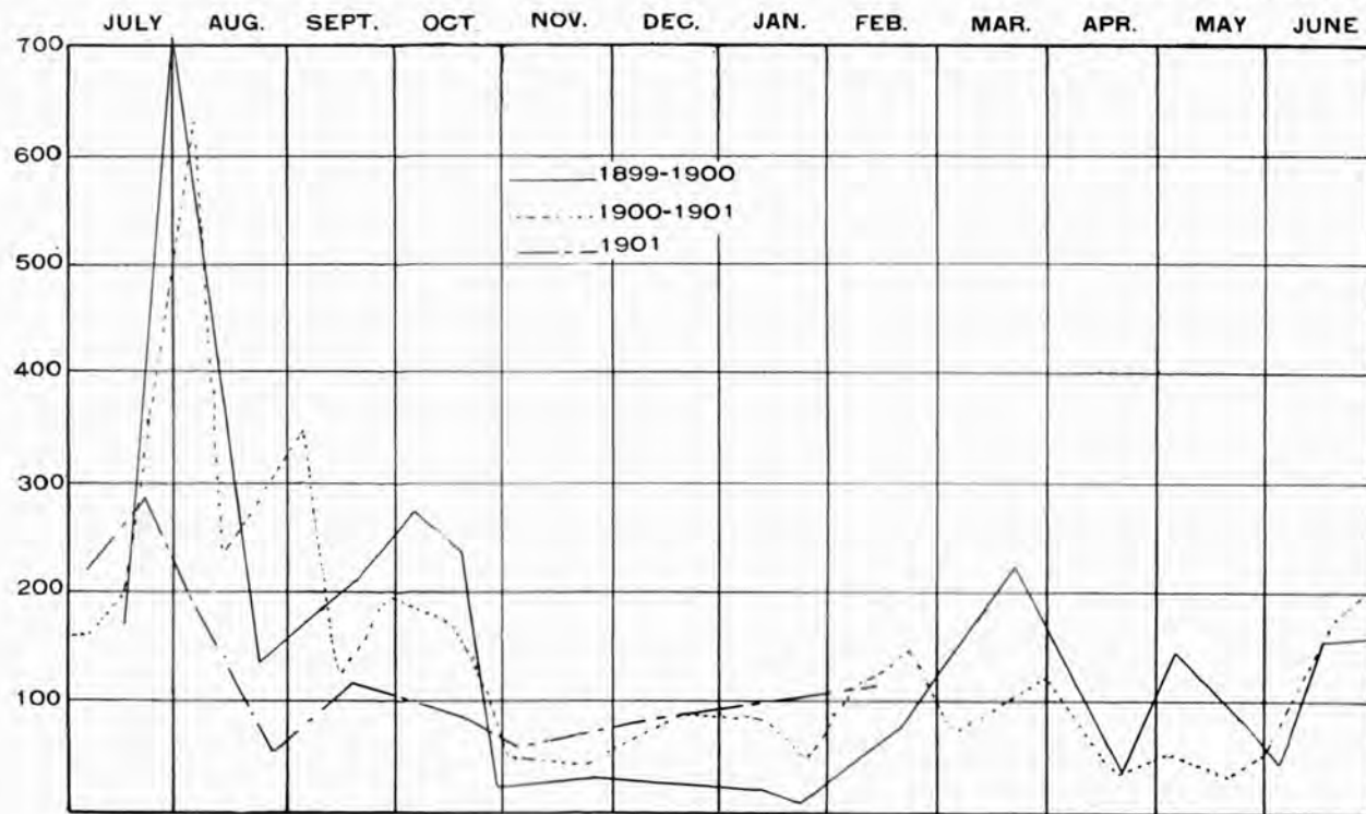
Curves of annual distribution of Diaptomus scellus and Diaptomus minutus per square meter in Green lake, the numbers being reckoned in thousands.
