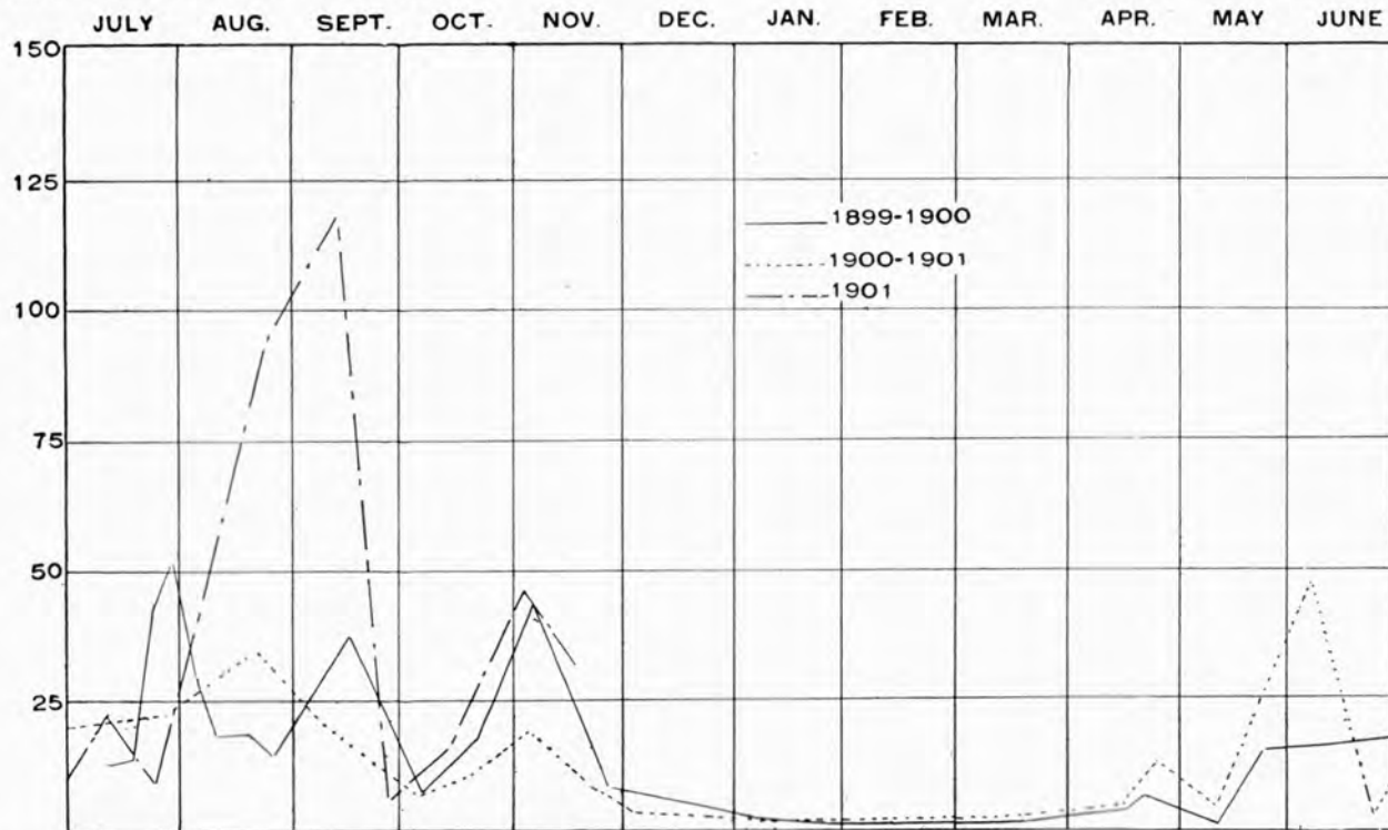
Curves of annual distribution of Diptomus oregonensis per square meter in Lake Winnebago, the numbers being reckoned in thousands.
